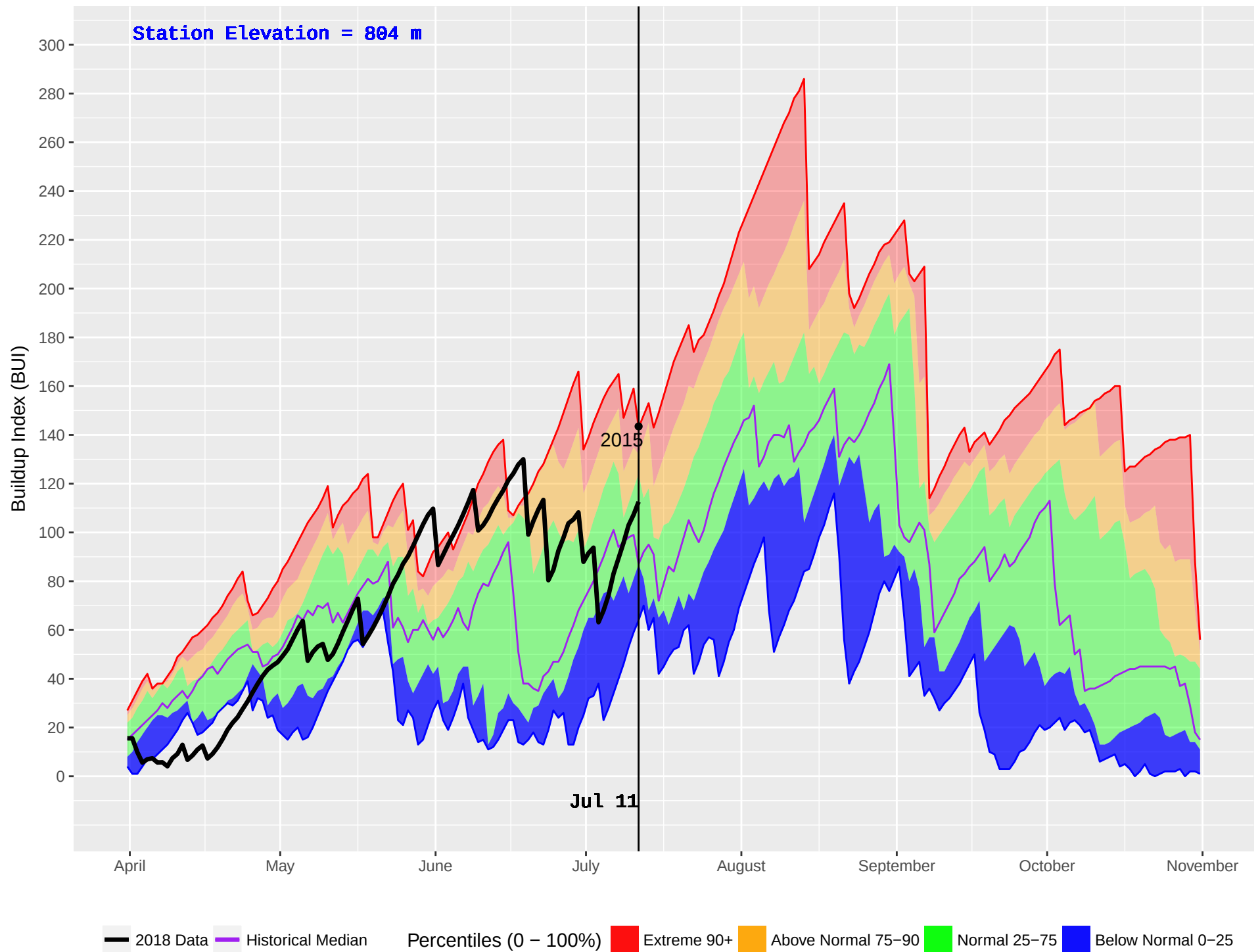
KOOCANUSA (1075) : Historical (2010–2016) and Current (2018) Noon Buildup Index (BUI)
