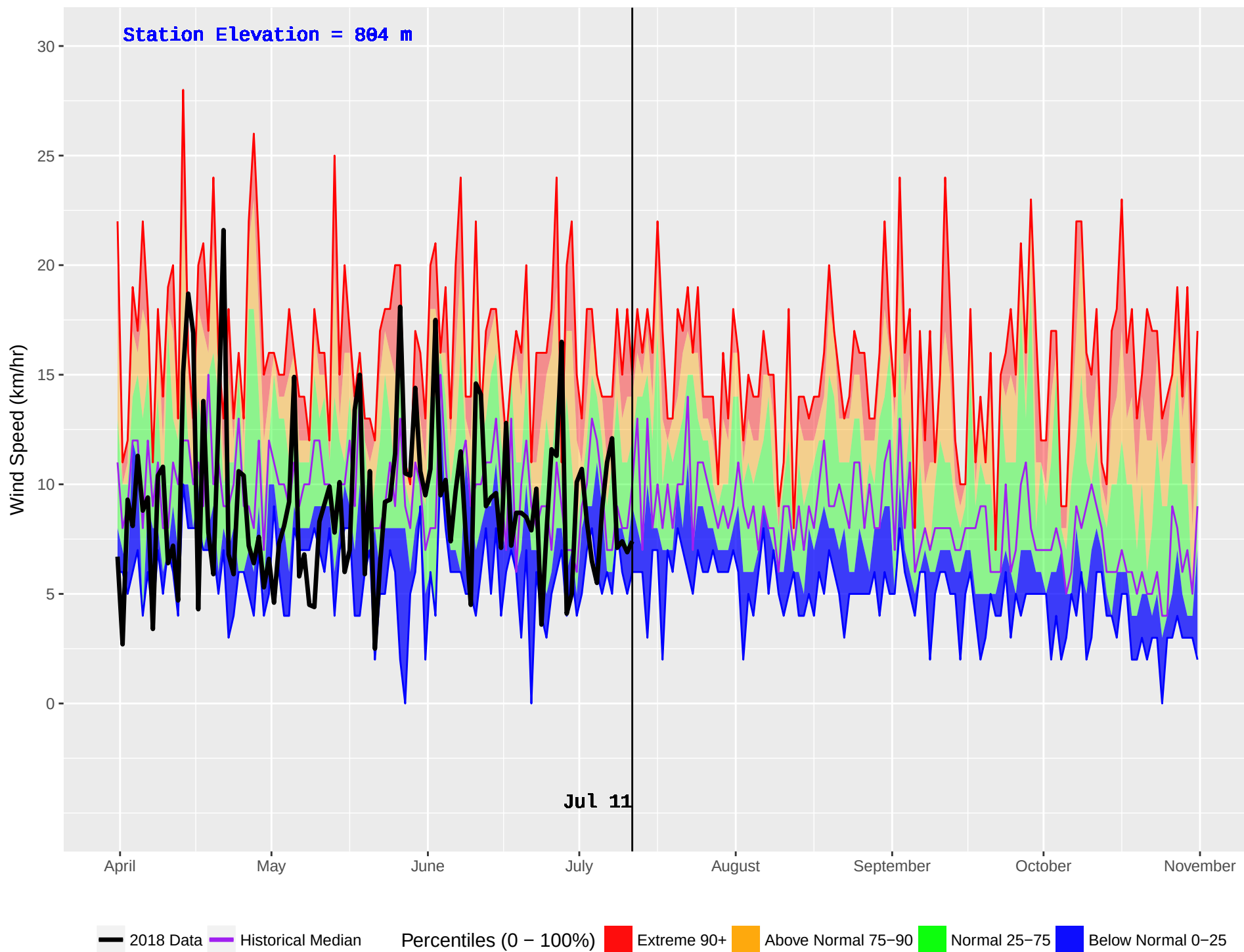
KOOCANUSA (1075) : Historical (2010–2016) and Current (2018) Noon Wind Speed
