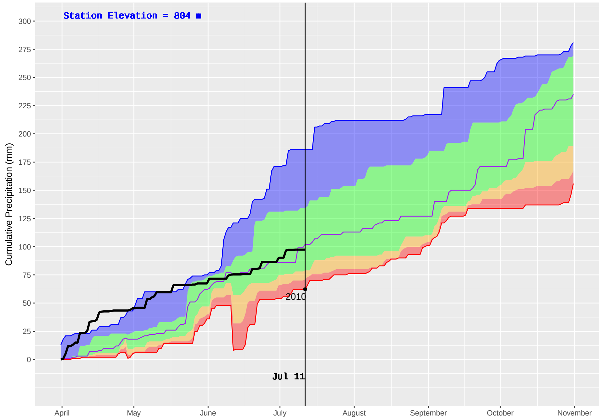
KOOCANUSA (1075) : Historical (2010–2016) and Current (2018) Noon Cumulative Precipitation
