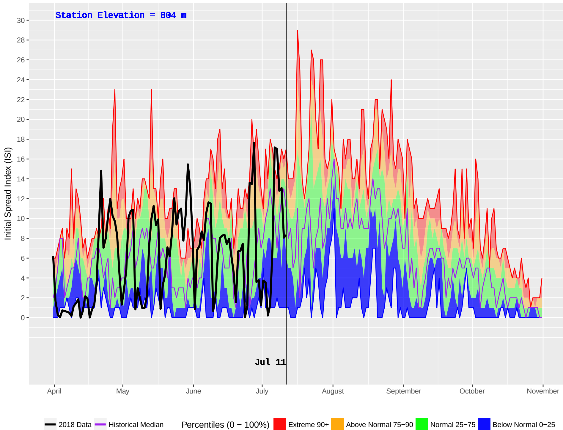
KOOCANUSA (1075) : Historical (2010–2016) and Current (2018) Noon Initial Spread Index (ISI)
