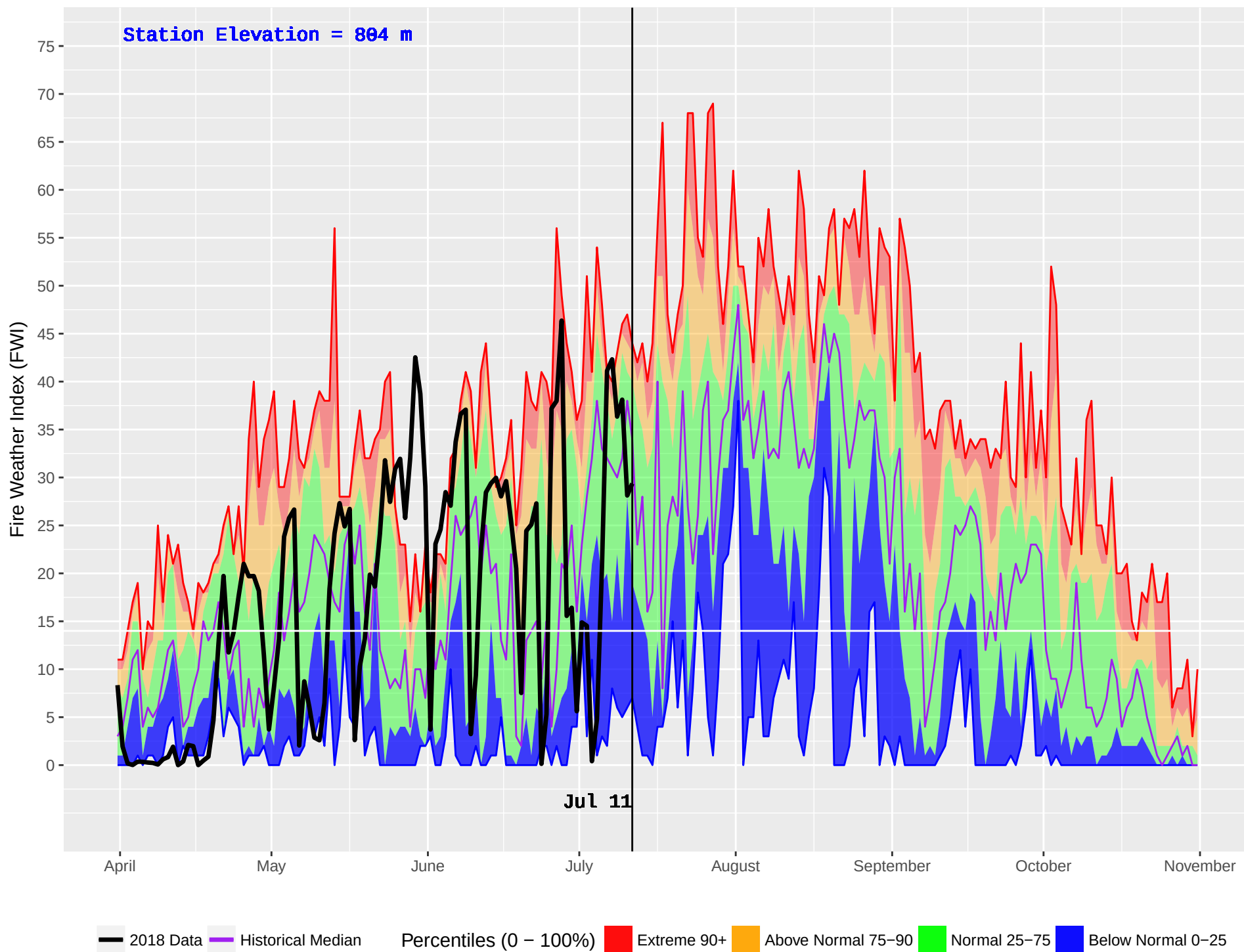
KOOCANUSA (1075) : Historical (2010–2016) and Current (2018) Noon Fire Weather Index (FWI)
